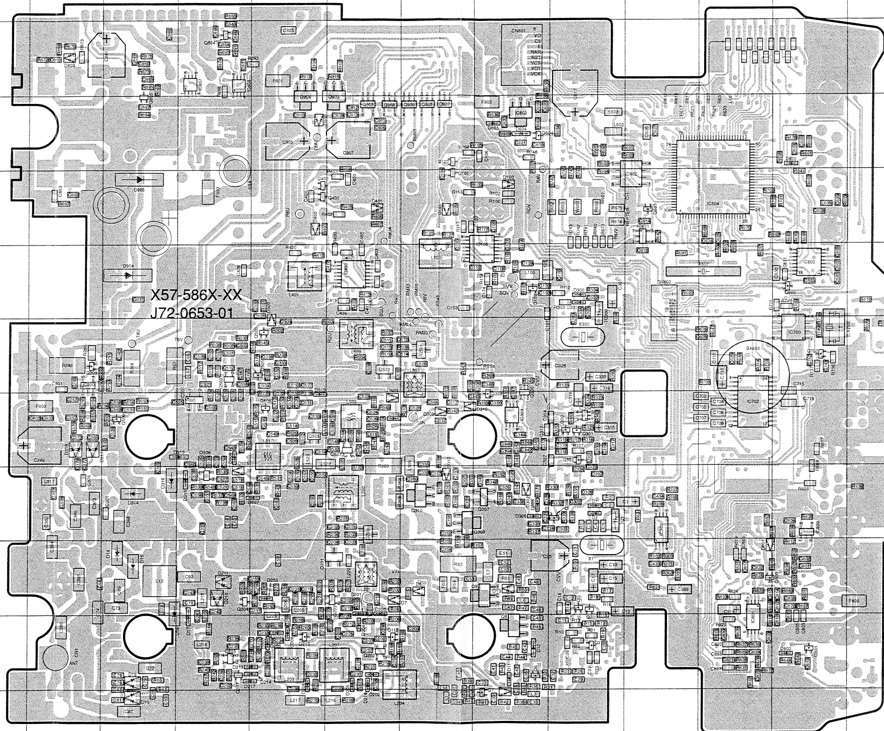
TX-RX UNIT (X57-586X-XX) Foil side view
