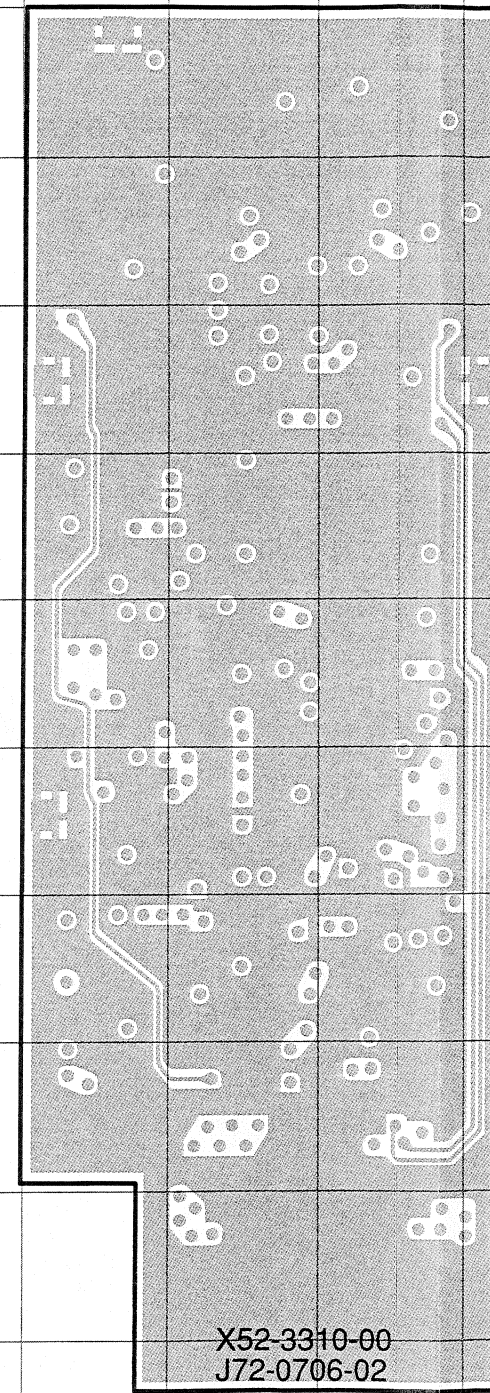
Component side Pattern 1 Pattern 2 Pattern 3 Pattern 4 Foil side
