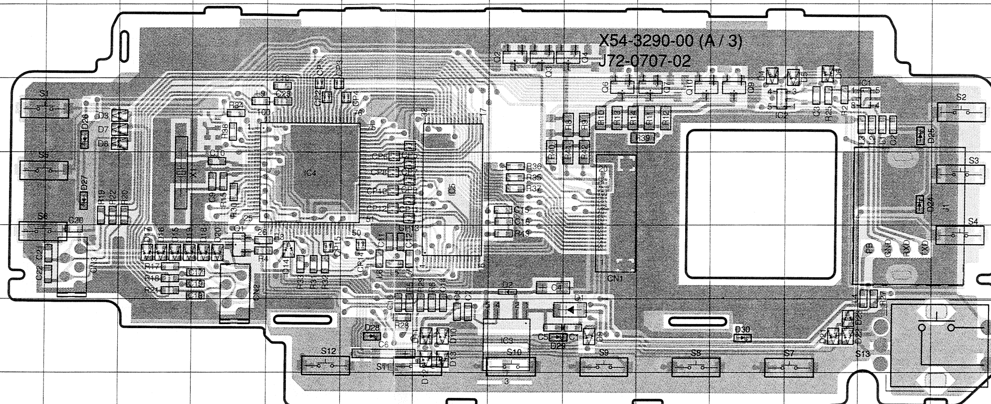
PANEL UNIT (X54-3290-00) Foil side view
