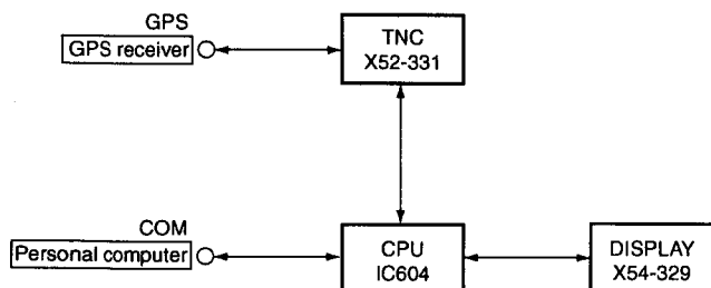
Fig.13 Structure of non-synchronized serial communication
